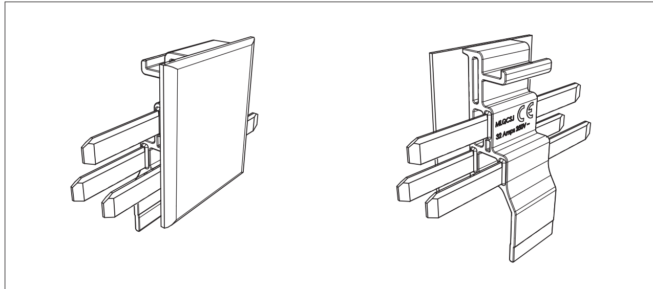
PERSPECTIVE VIEWS
