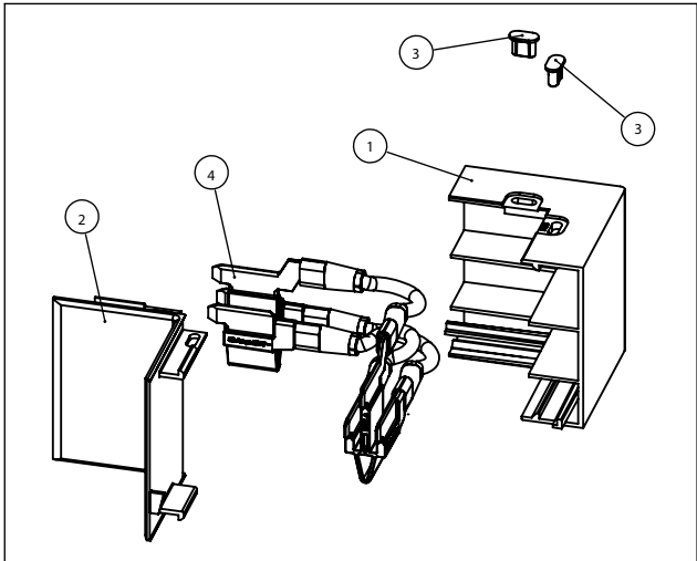
EXPLODED VIEW
